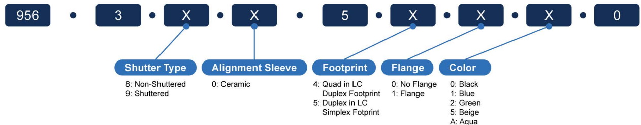
LC Singlemode Duplex Adapter Low Profile
